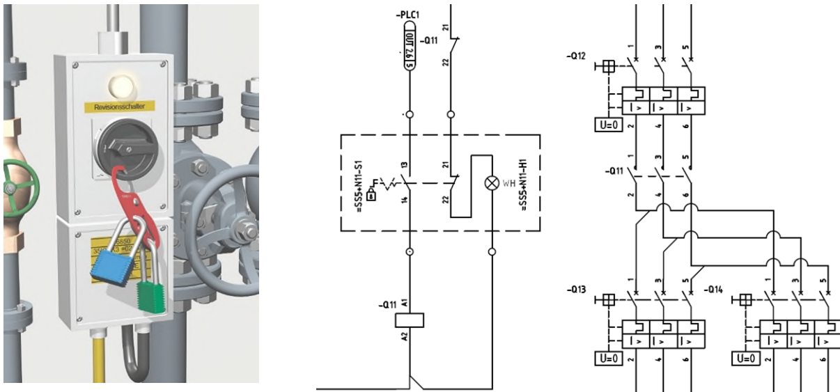
Figure 2: Maintenance switch, operating indirectly with signal lamp
